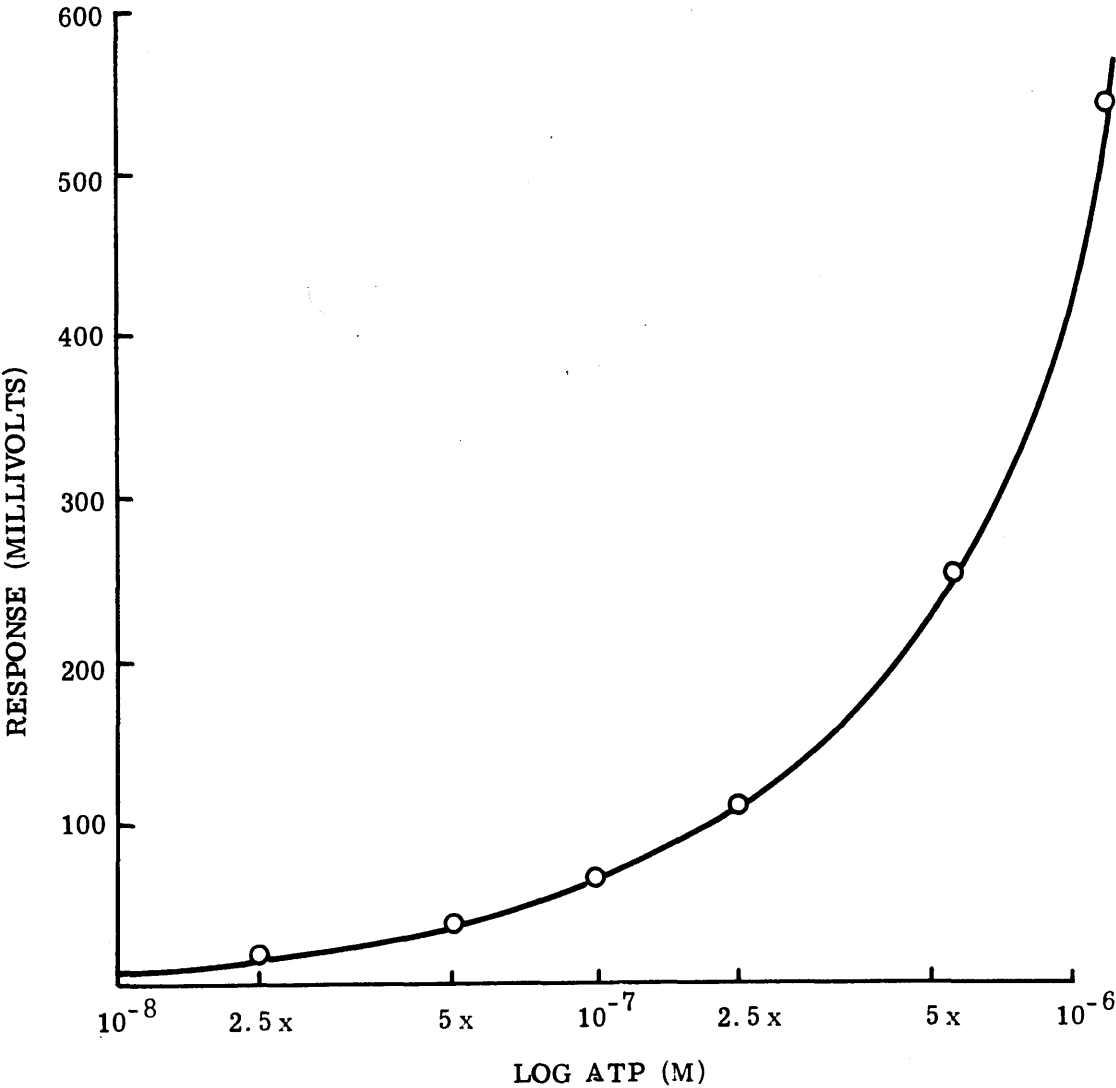
TYPICAL DOSE RESPONSE CURVE FOR ATP
