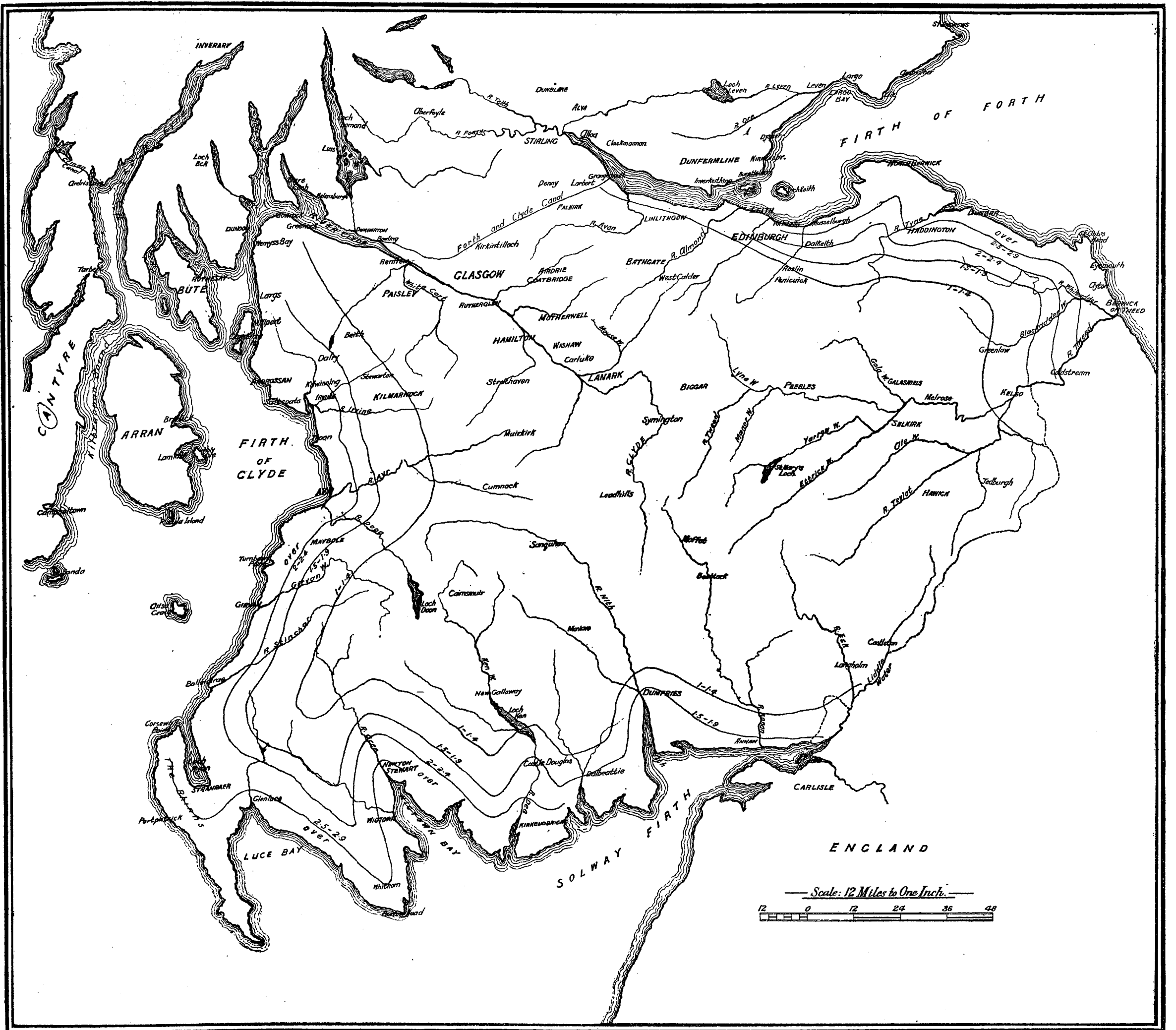
Map 3.—AREAS OF EQUAL CHLORINE CONTENT.
