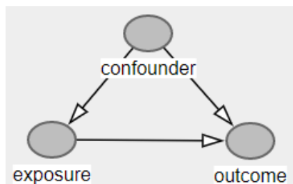
Figure 2-5: A confounder
