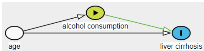
Figure 2-8: Adjusted confounder in DAGitty
