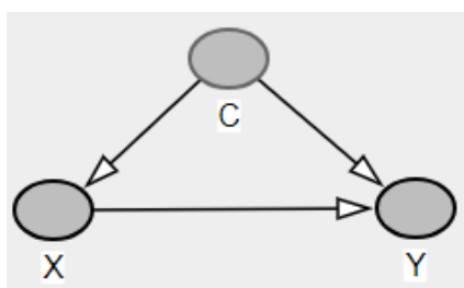
Figure 8-5: Exposure mediates the effect of the confounder on the outcome
