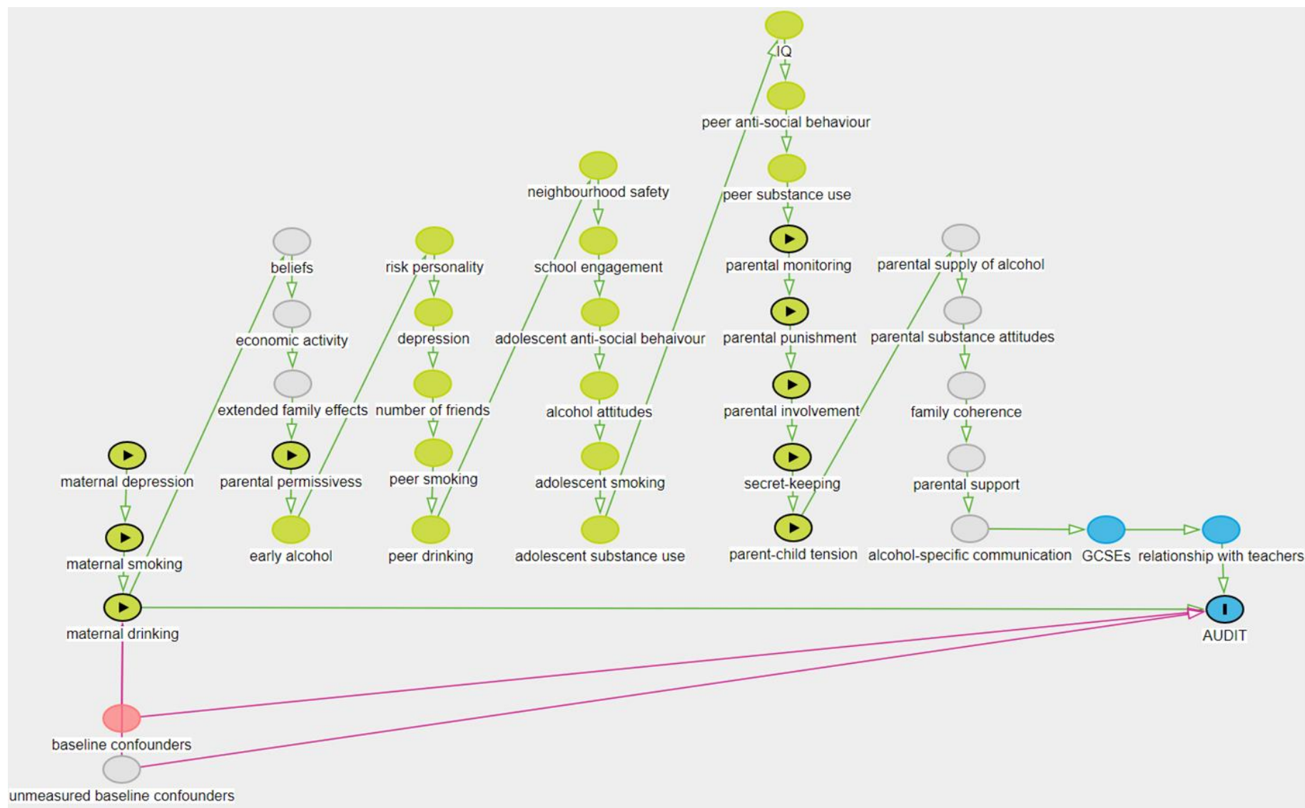
Figure 7-7: Further simplification of data I-DAG
