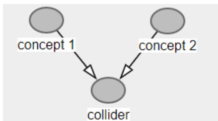
Figure 2-9: A collider
