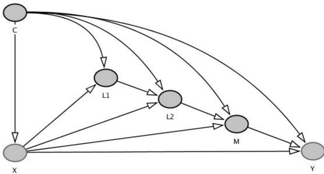
Figure 3-4: Mediation model with two variables in L
