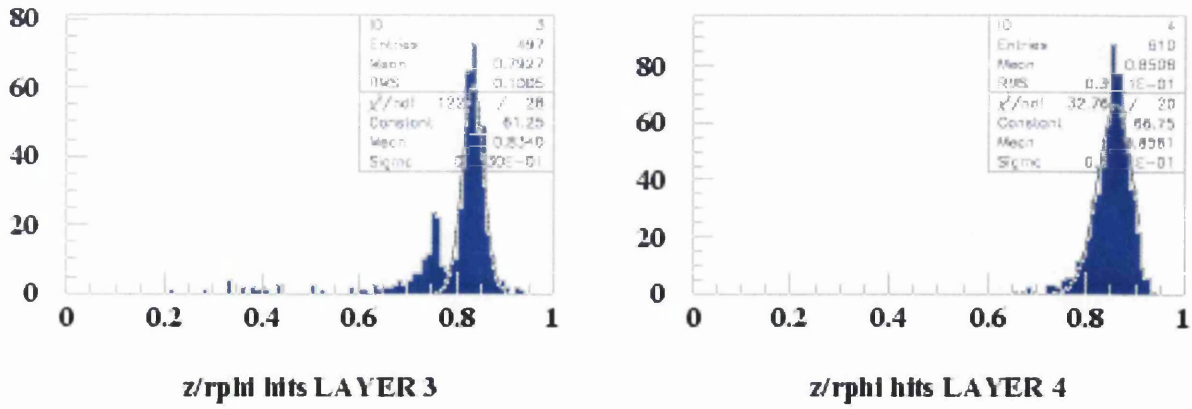
Figure A.1: Number of clusters associated with tracks on one side of the silicon divided by the number on the other side for SVXII layers three and four of the central barrel. The secondary, lower, peak in the layer 3 plot is due to ladders which have a lower efficiency since the ladder in the next radial layer is switched off.
