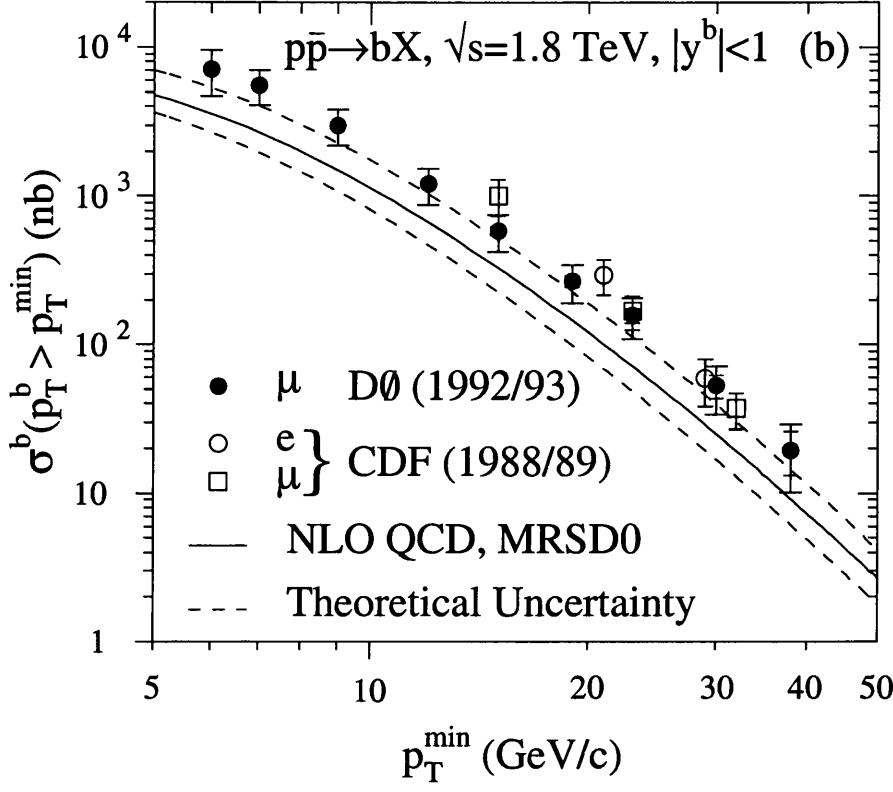
Figure 1.9: b quark production cross section as a function of p_T [25].
