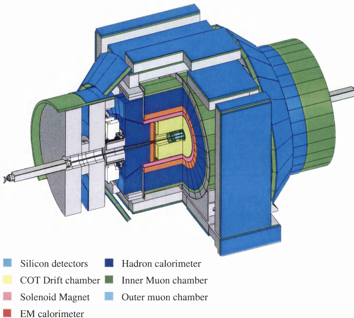
Figure 2.2: The 5000ton CDF detector.
