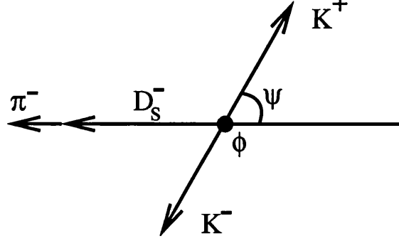
Figure 3.3: The helicity angle is defined as the angle between the K^+ and D_s^- in the rest frame of the \phi meson.
